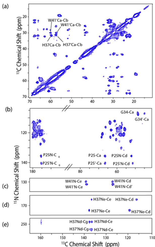
Figure 2. (a) Two-dimensional ^{13}\text{C} – ^{13}\text{C} 20 ms PDSO of M2 18–60 H57Y ILFY (CP contact time 1.5 ms and 83 kHz TPPM decoupling) and (b) 2D ^{13}\text{C} – ^{15}\text{N} 3.2 ms ZF-TEDOR of M2 18–60 H57Y ILFY both acquired at \omega_r/2\pi = 12.5 kHz 700 MHz ^1\text{H} frequency, pH 7.5, and -6 °C. (c–e) Strips showing aromatic regions of the ZF-TEDOR. This data shows peak doubling indicative of dimer of dimer structure, even after protonation has partially occurred.
